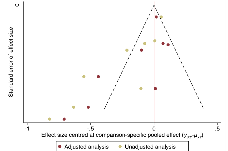
Figure S5. Funnel plot for comparison-specific cross-sectional pooled effect sizes for attention.
