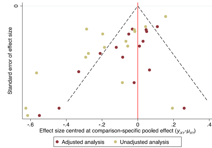
Figure S4. Funnel plot for comparison-specific cross-sectional pooled effect sizes for memory.
