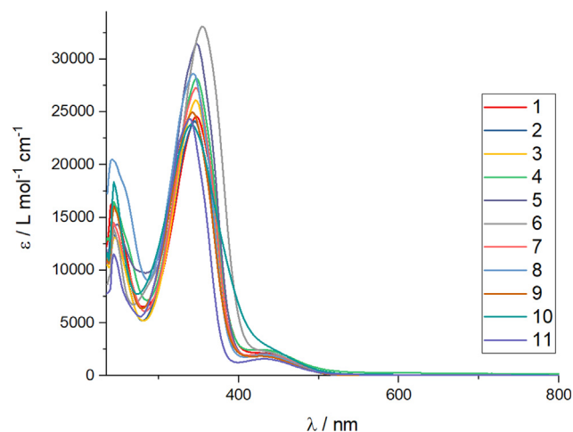
Fig. 3 UV-vis in \text{CH}_3\text{Cl} for 1–11.
