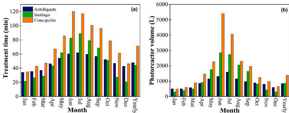
Fig. 6. (a) Estimation of the treatment time needed to reach 75 % degradation of paracetamol polluted water, (b) Estimation of the photo reactor volume needed to treat 10 \text{ m}^3 \text{ day}^{-1} of polluted water based on UVR and temperature monthly and yearly average values got from the TMY.
