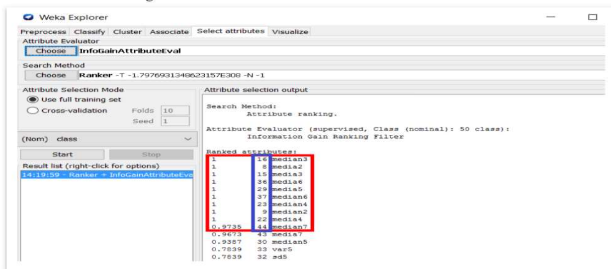
Figure 6. Visual interface of attribute selection in WEKA
