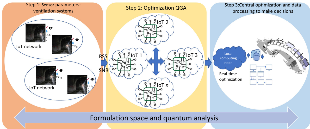
Fig. 10 QGA conceptual model
