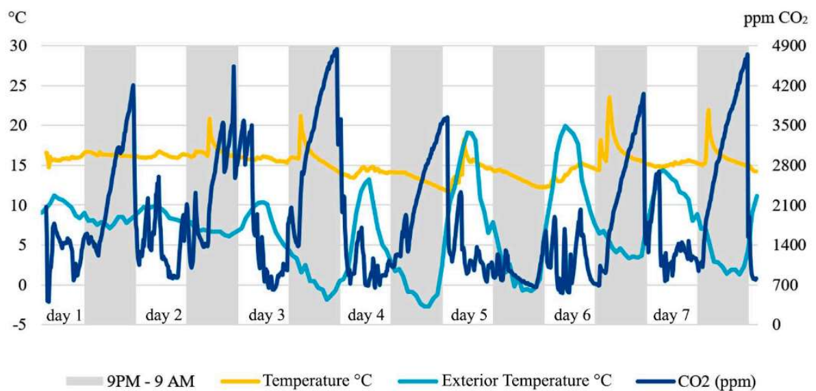
Figure 9. Temperature and CO 2 concentration graph. Case 2: bedroom located on second floor, with poor ventilation conditions. Records of June 24 through July 1, 2021.
