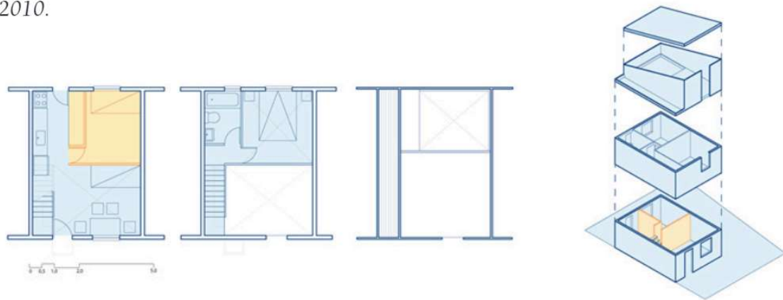
Figure 3. Stage I, corresponding to the original state. Isometric of a housing type delivered in 2010.
