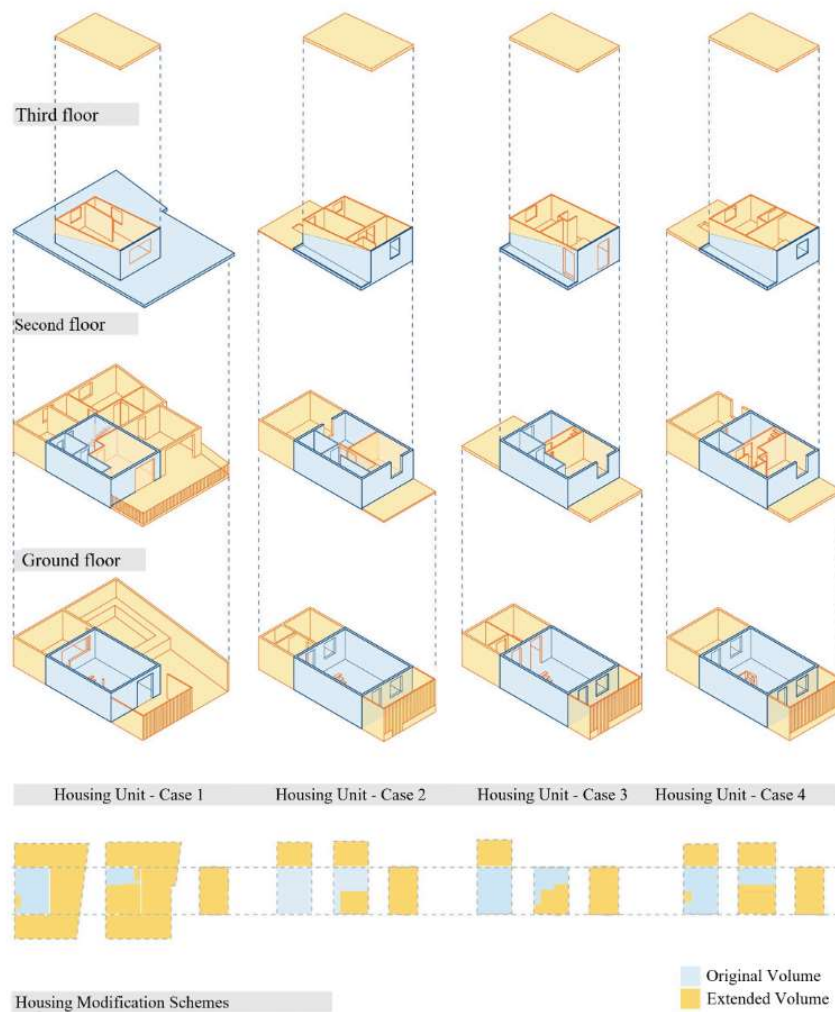
Figure 5. Stage III, corresponding to the present state of the four houses, incorporating the modifications carried out by the residents themselves.
