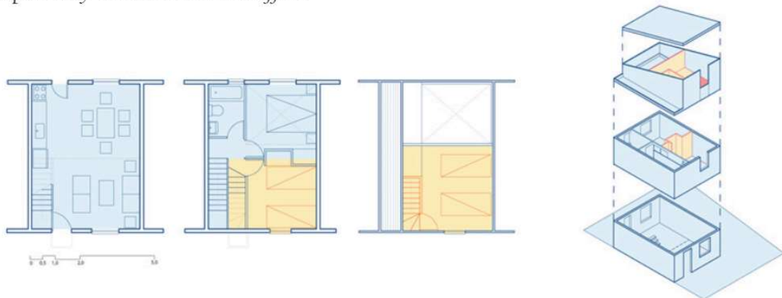
Figure 4. Stage II, corresponding to what was designed. Isometric of the house with modifications proposed by the architectural office.
