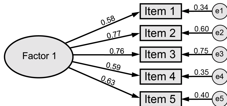
Figure 1. Factorial structure.
